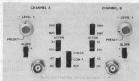
Figure 1. Input Switches
