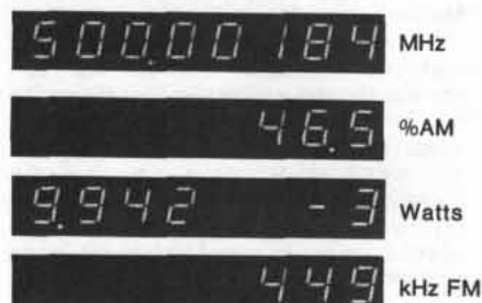
Modulation Analyzer displays of RF signal parameters.
