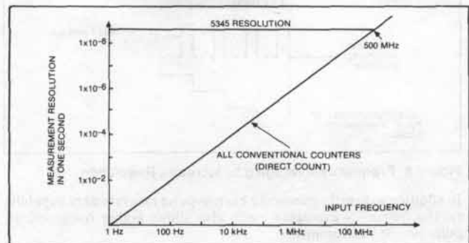
Figure 3. Measurement Resolution
